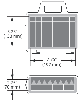
= Foam cradled dimensions
